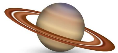
Saturn
